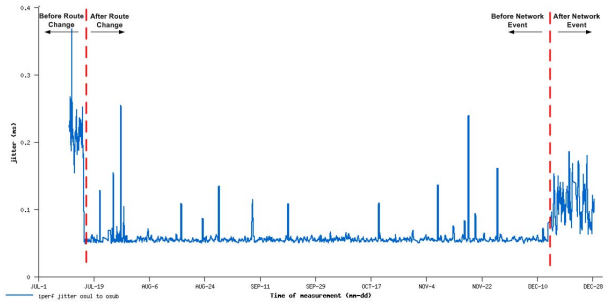
Fig. 10. Jitter measurements along Campus Network Backbone Path
