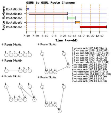
Fig. 5. Route Changes along Campus Network Backbone Path
