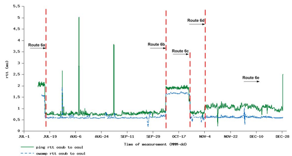
Fig. 6. Delay measurements along Campus Network Backbone Path
