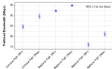
Fig. 9. Mean and 95% CI Plot for Bandwidth measurements
