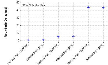
Fig. 7. Mean and 95% CI Plot for Delay measurements
