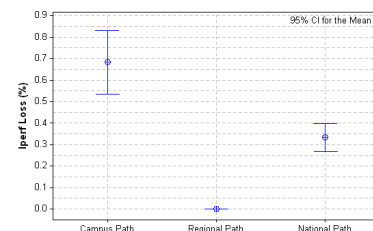
Fig. 12. Mean and 95% CI Plot for Loss measurements
