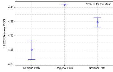
Fig. 13. Mean and 95% CI Plot for MOS measurements
