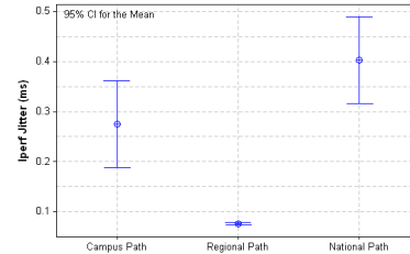
Fig. 11. Mean and 95% CI Plot for Jitter measurements
